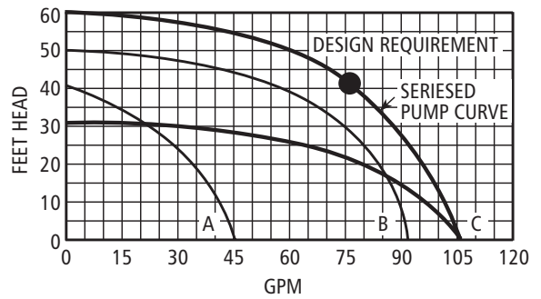
Seriesed Pump Curve Figure 34
