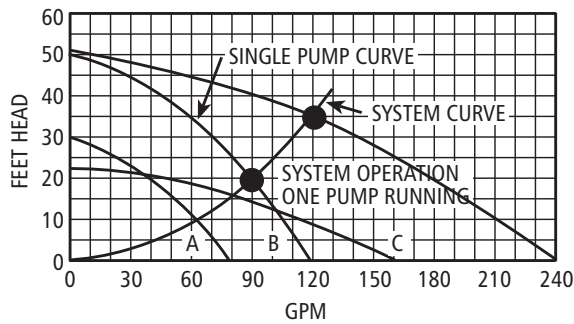
Single Pump Operation Figure 24
