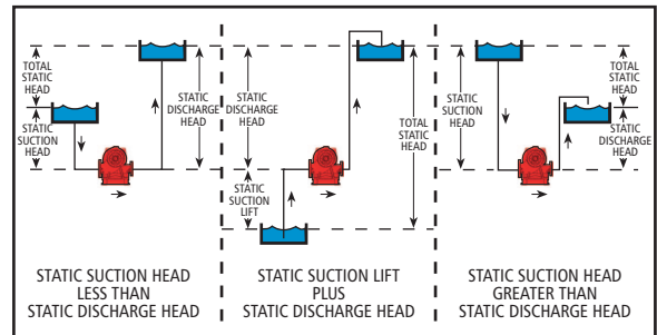
Open System Definitions Figure 16
