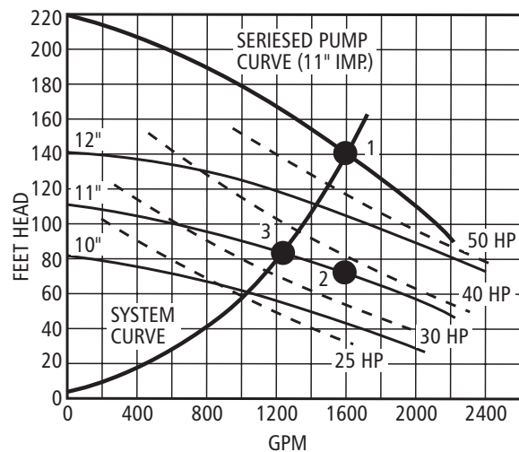
Seriesed Pump Operation Figure 37
