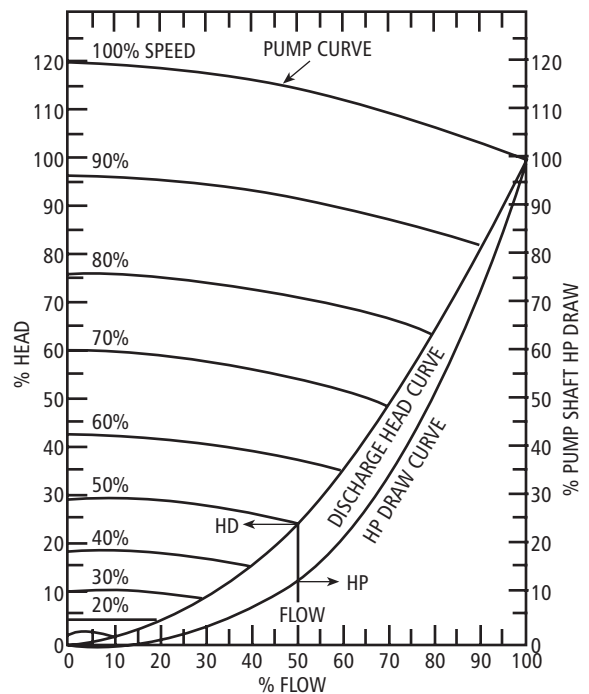
Theoretical Relationship Among Speed, Flow, and Head Figure 40
