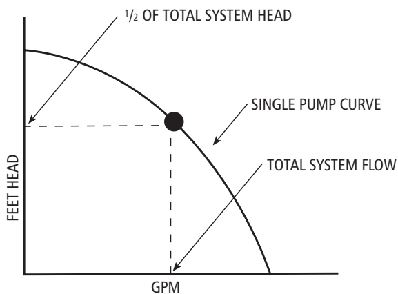
Basic Series Pump Operation Figure 29
