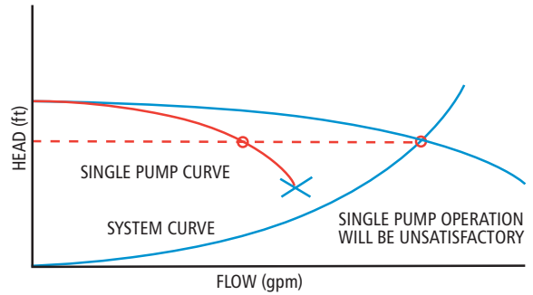
Unsatisfactory Single Pump Operation Figure 12
