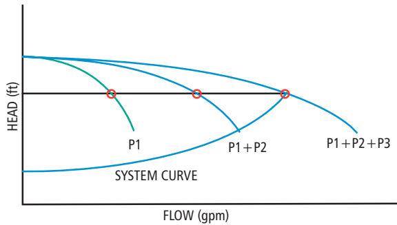
Three Parallel Pumps; Open System Figure 18
