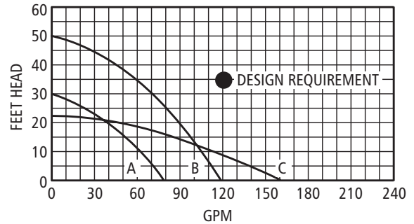
Typical Small Pump Curves Figure 21
