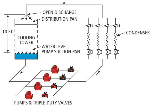
Typical Large Condenser Water System Figure 17
