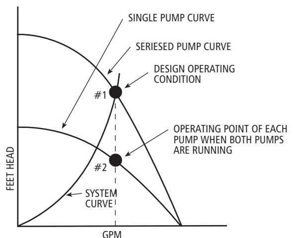
Seriesed Pump - System Operation Figure 31
