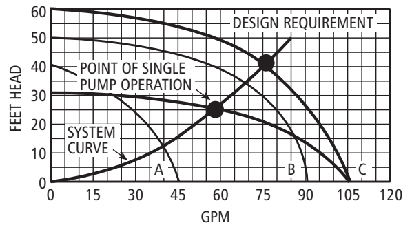
Single Pump Operation Figure 35
