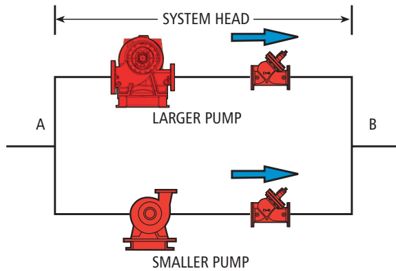
Dis-similar Pumps in Parallel Figure 14
