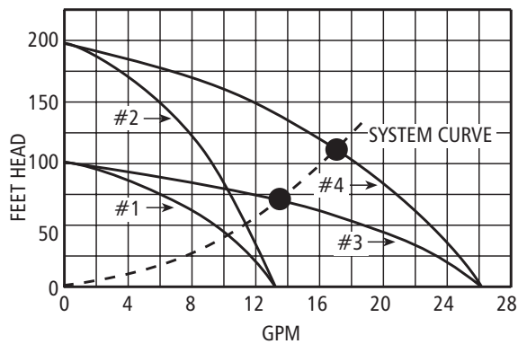
Combination Parallel & Series Pump Curves Figure 39
