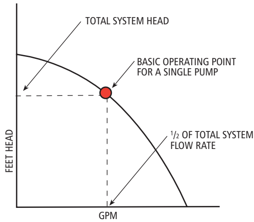
Basic Paralleled Pump Operating Point Figure 2
