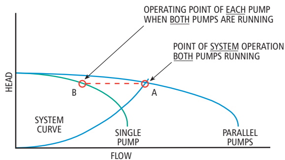
Paralleled Pump System Operation Figure 8
