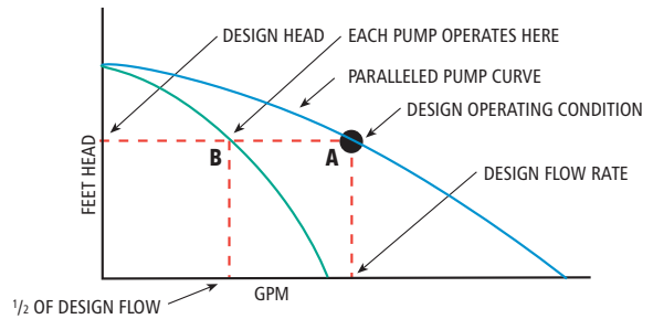
Two Parallel Pump System Operation Figure 4
