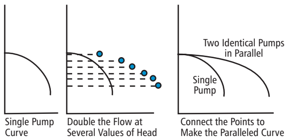
Two Identical Pumps Paralleled Pump Curve Construction Figure 3
