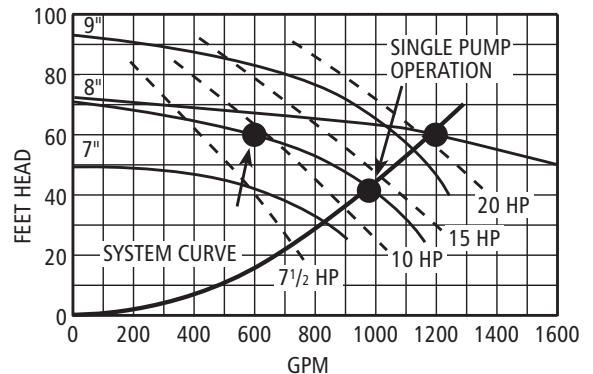
Single Pump Operation Figure 27
