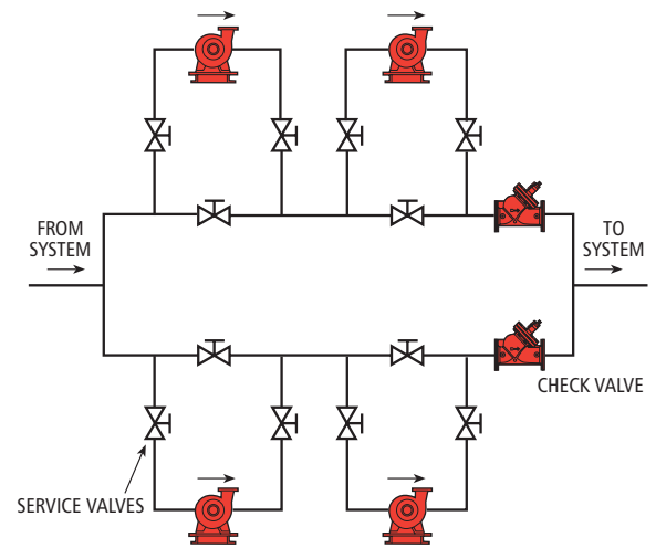
Basic Paralleled & Seriesed Pump Installation Figure 38
