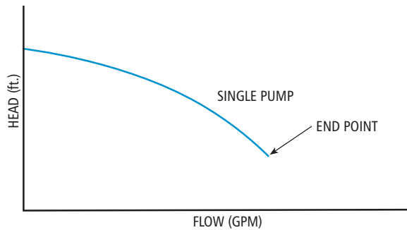
Pump Curve End Point Figure 11
