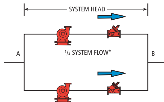
Basic Parallel Pump Installation Figure 1
