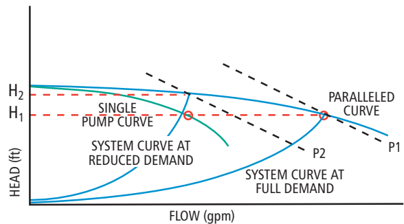
System at Part Load Figure 19
