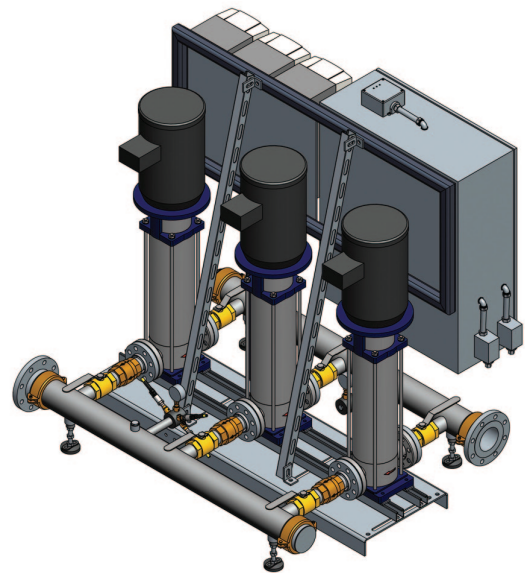
Parallel, Multistage Domestic Water System Pump Package Figure 42
