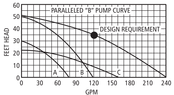
Paralleled "B" Pump Curve Figure 22
