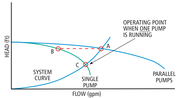
Single Pump Operation - Paralleled Installation Figure 9
