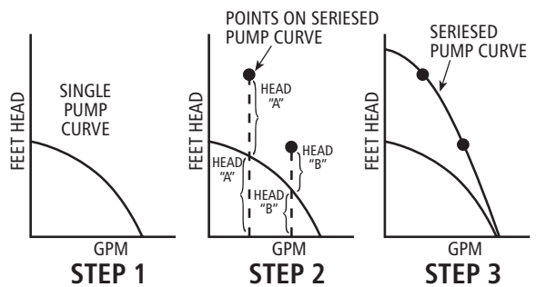
Seriesed Pump Curve Construction Figure 30
