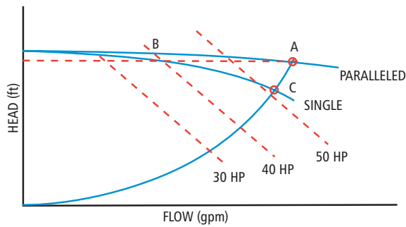
BHP Increase During Single Pump Operation Figure 10
