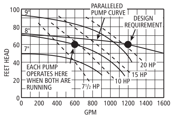
Paralleled Pump Curve Figure 26
