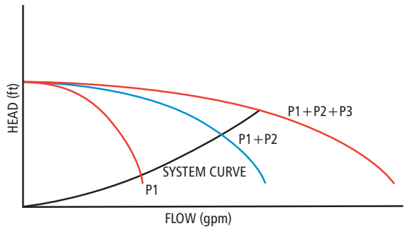
Three Pump Paralleled Pump Curve Construction Figure 13
