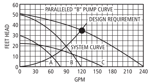
System Curve Figure 23
