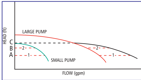
Small Lower Head Pump; "Piggybacks" its Flow-Head Curve onto Larger Pump Figure 15
