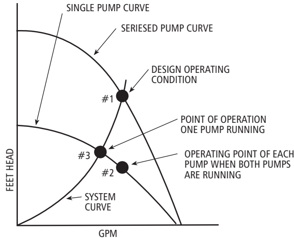
Single Pump Operation - Seriesed Installation Figure 32
