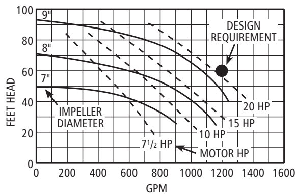
Typical Larger Pump Curves Figure 25
