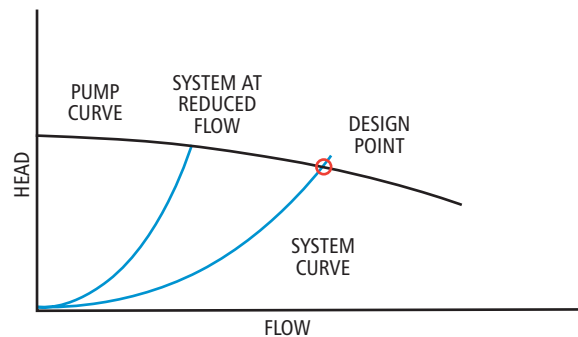
The System Curve Figure 7
