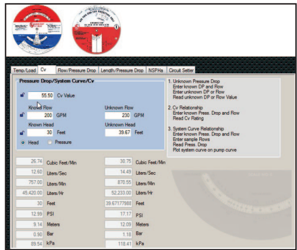
System Syzer ® System Curve Calculation Figure 6
